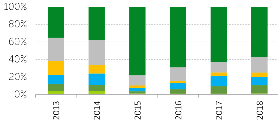
Equities
