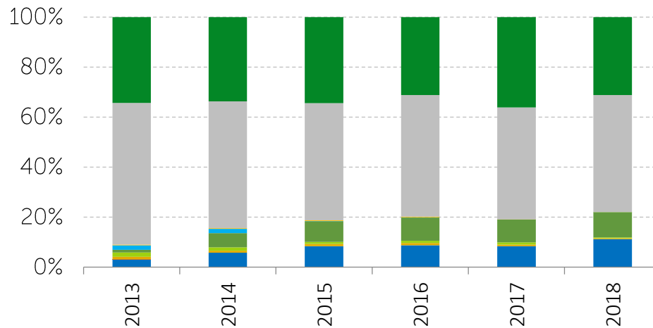
Corporate bonds
